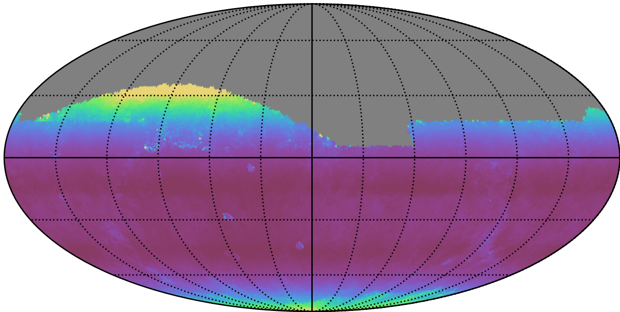
extra_ss_neo4_v3.4_10yrs Yr 1 all bands: Median airmass
