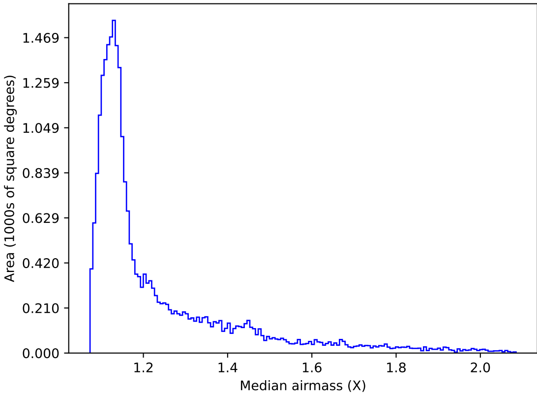
extra_ss_neo4_v3.4_10yrs Yr 1 all bands: Median airmass
