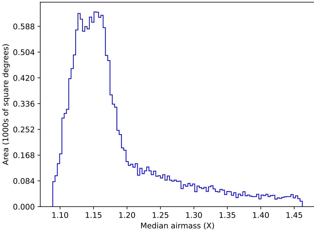
extra_ss_neo4_v3.4_10yrs WFD z band: Median airmass
