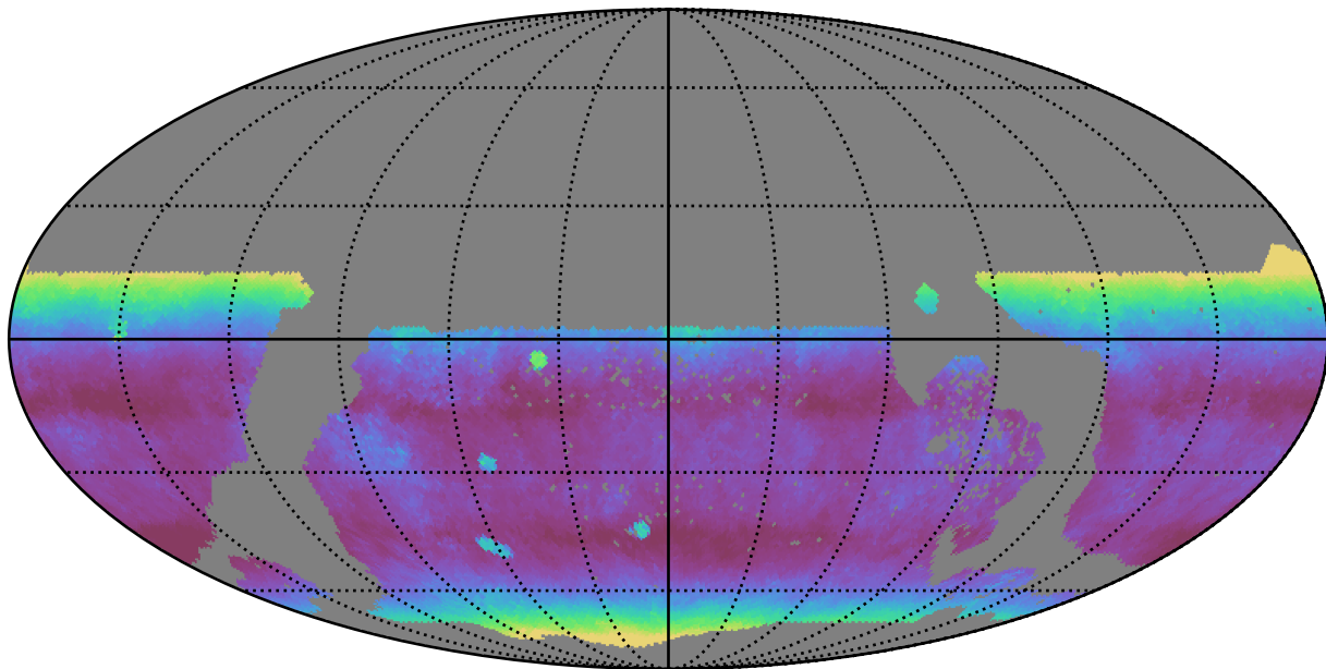
extra_ss_neo4_v3.4_10yrs WFD y band: Median airmass
