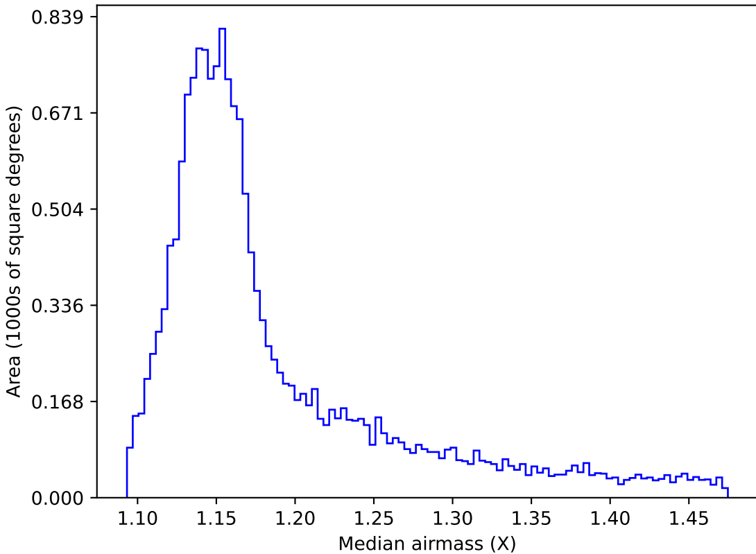
extra_ss_neo4_v3.4_10yrs WFD y band: Median airmass
