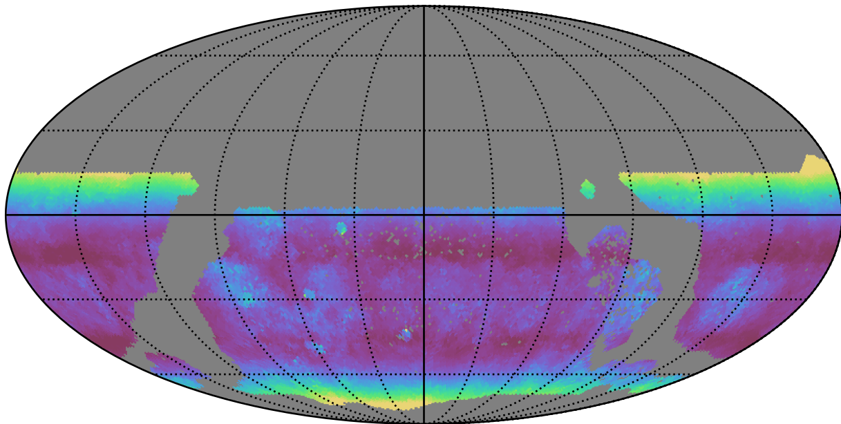
extra_ss_neo4_v3.4_10yrs WFD u band: Median airmass
