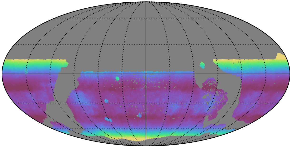
extra_ss_neo4_v3.4_10yrs WFD r band: Median airmass
