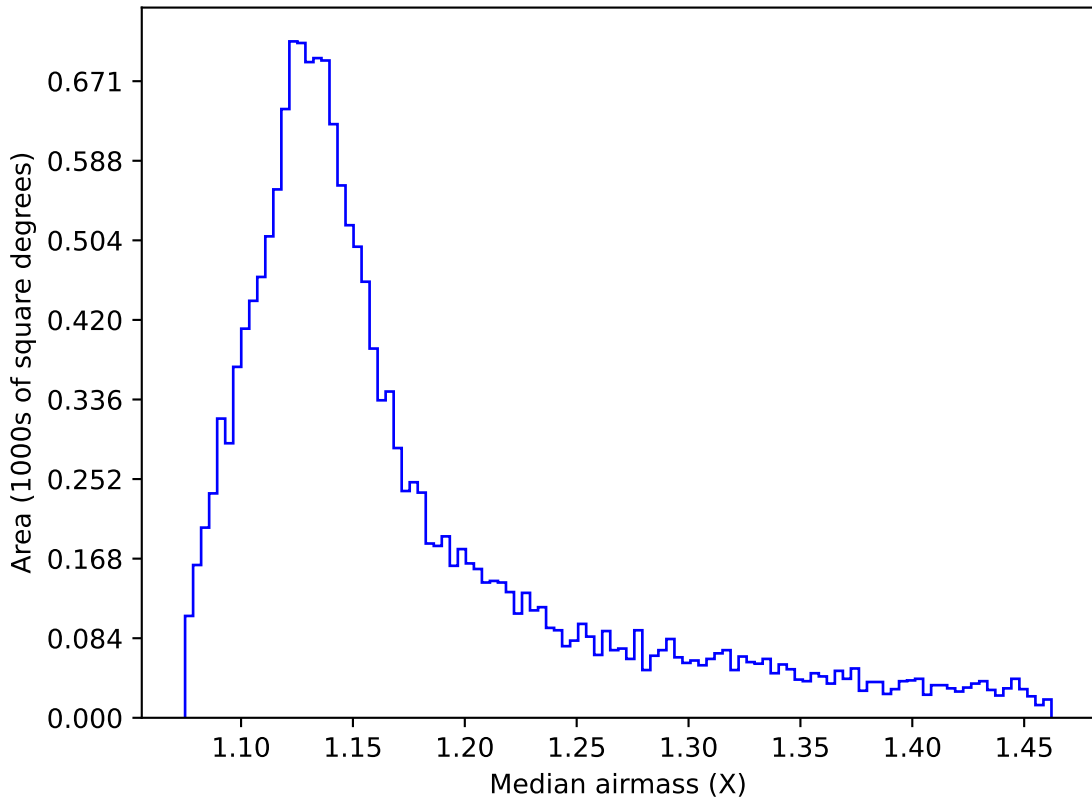
extra_ss_neo4_v3.4_10yrs WFD r band: Median airmass
