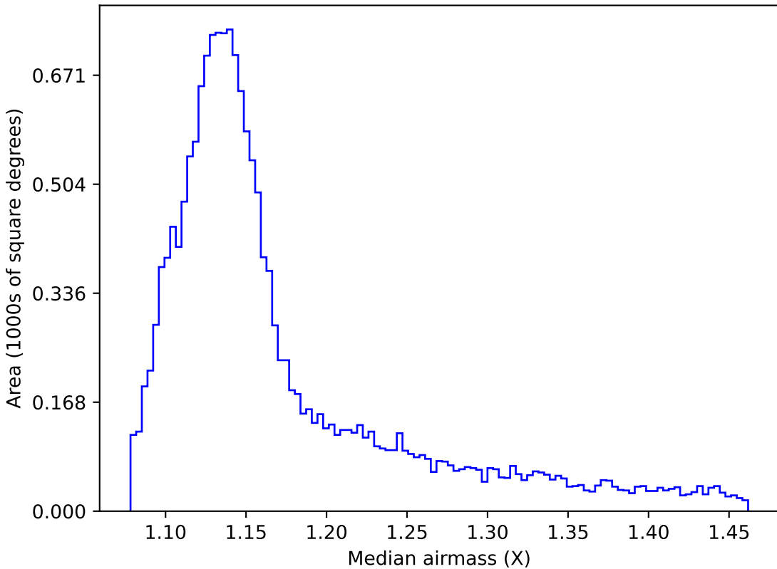
extra_ss_neo4_v3.4_10yrs WFD i band: Median airmass
