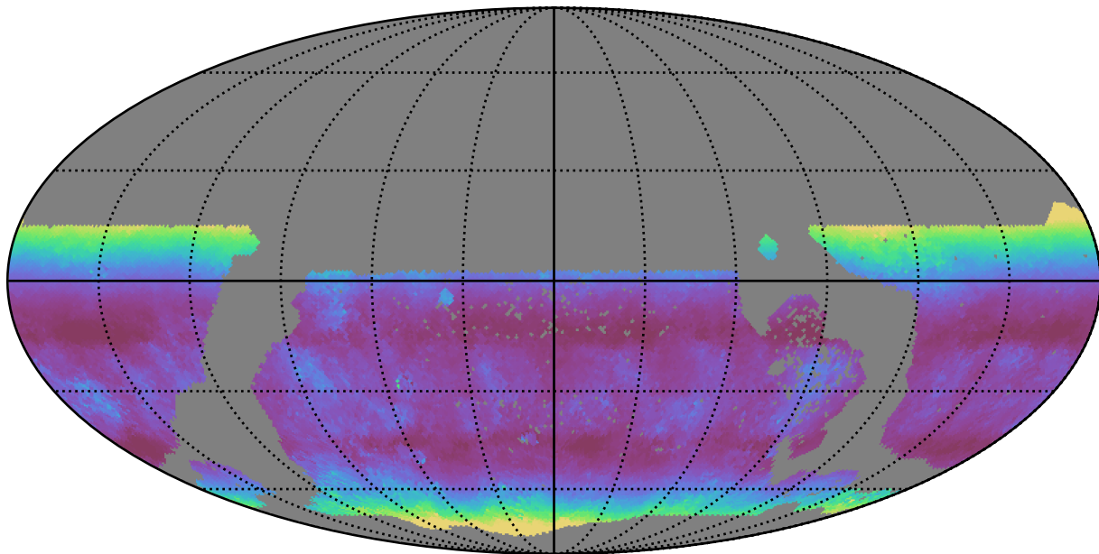
extra_ss_neo4_v3.4_10yrs WFD g band: Median airmass
