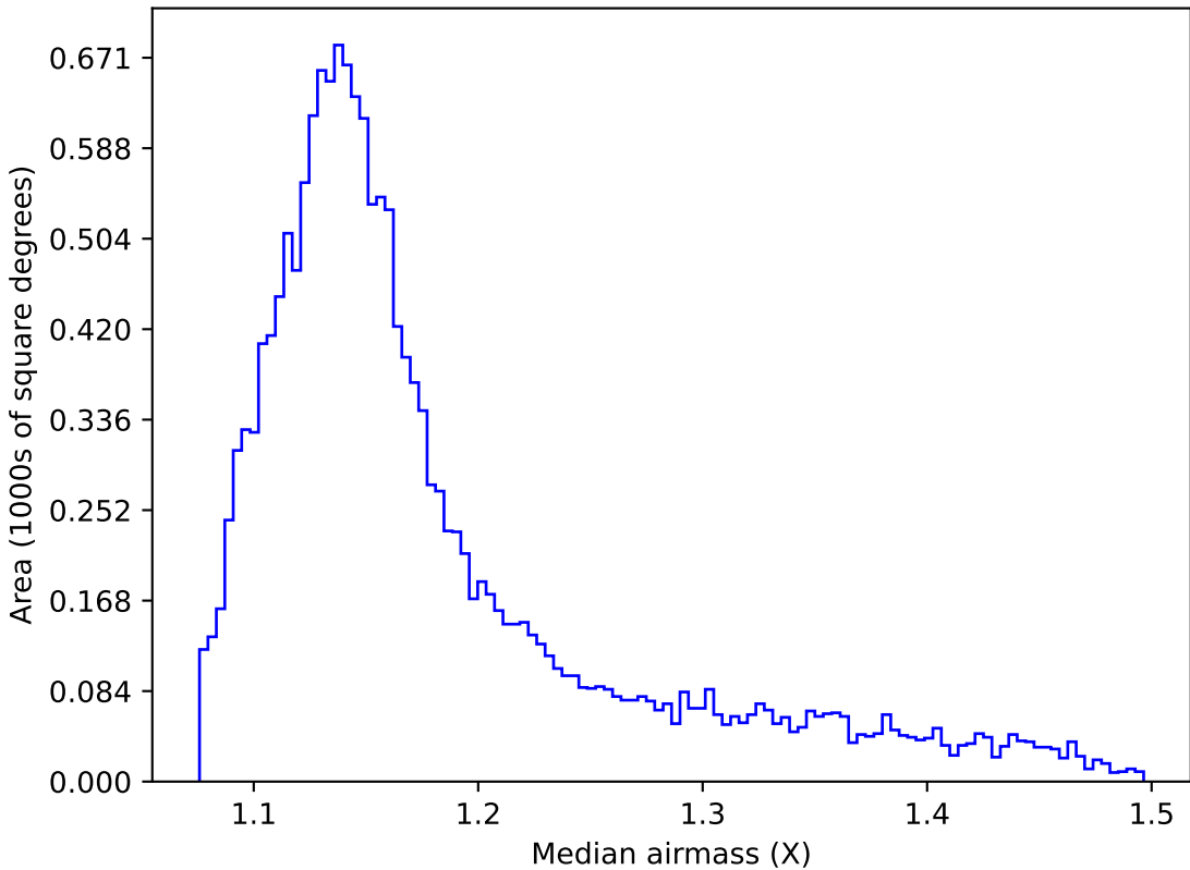
extra_ss_neo4_v3.4_10yrs WFD g band: Median airmass
