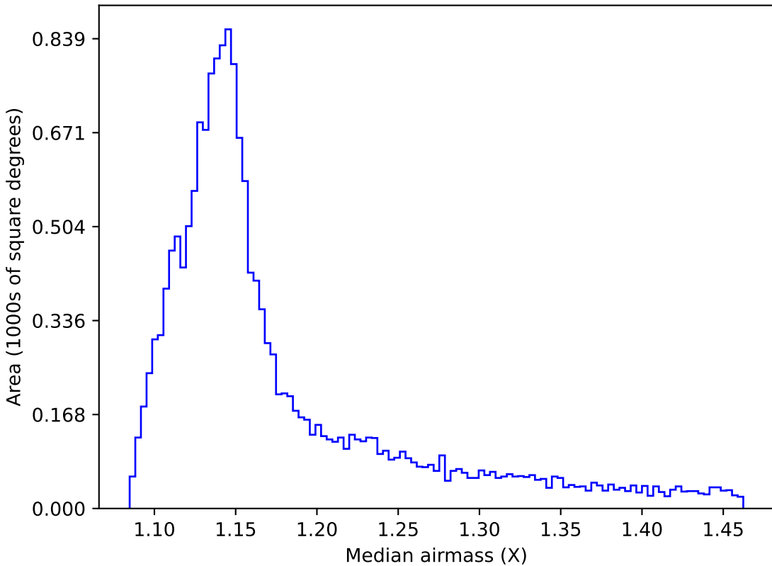
extra_ss_neo4_v3.4_10yrs WFD all bands: Median airmass
