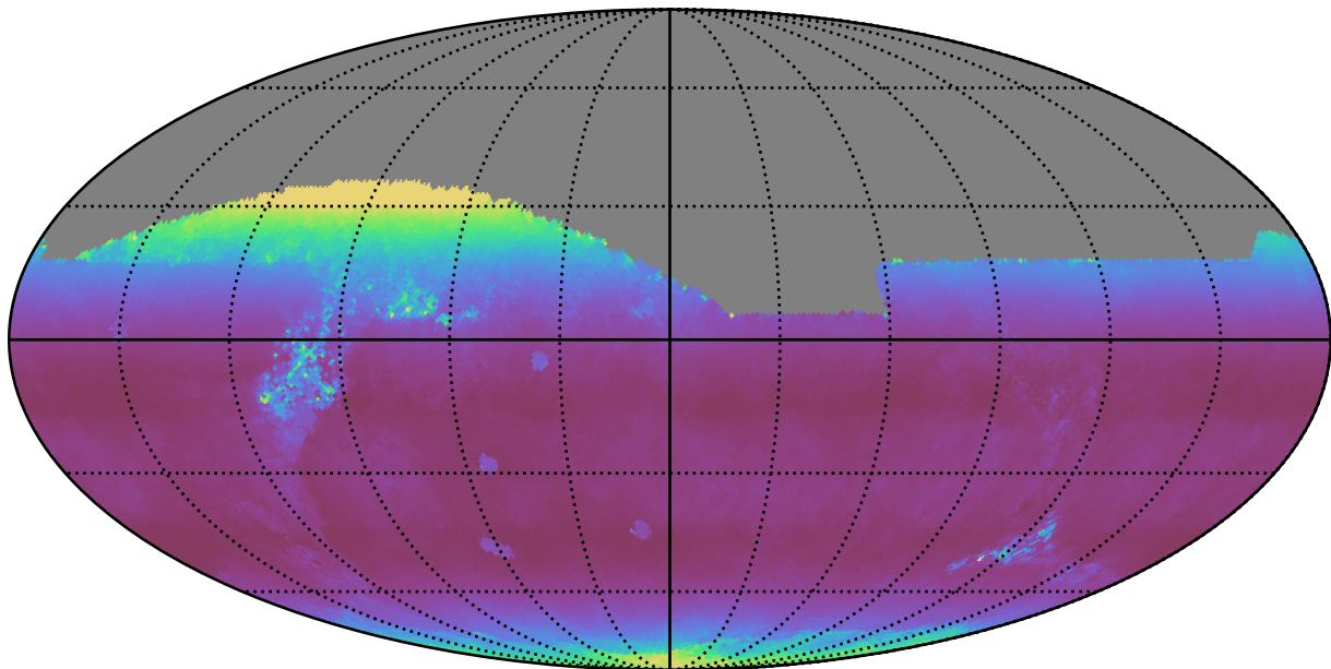
extra_ss_neo4_v3.4_10yrs All sky z band: Median airmass
