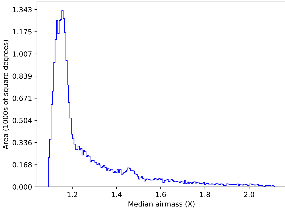
extra_ss_neo4_v3.4_10yrs All sky z band: Median airmass
