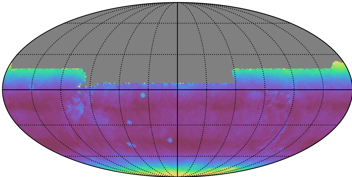
extra_ss_neo4_v3.4_10yrs All sky y band: Median airmass
