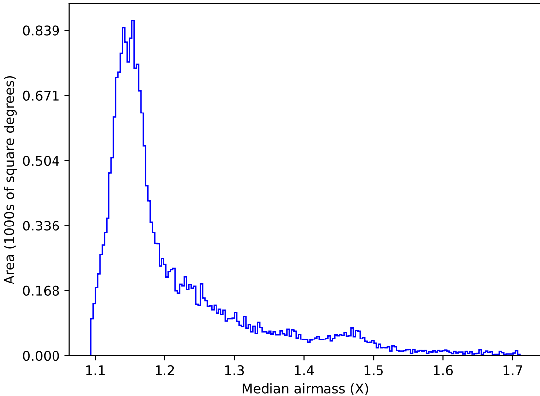
extra_ss_neo4_v3.4_10yrs All sky y band: Median airmass
