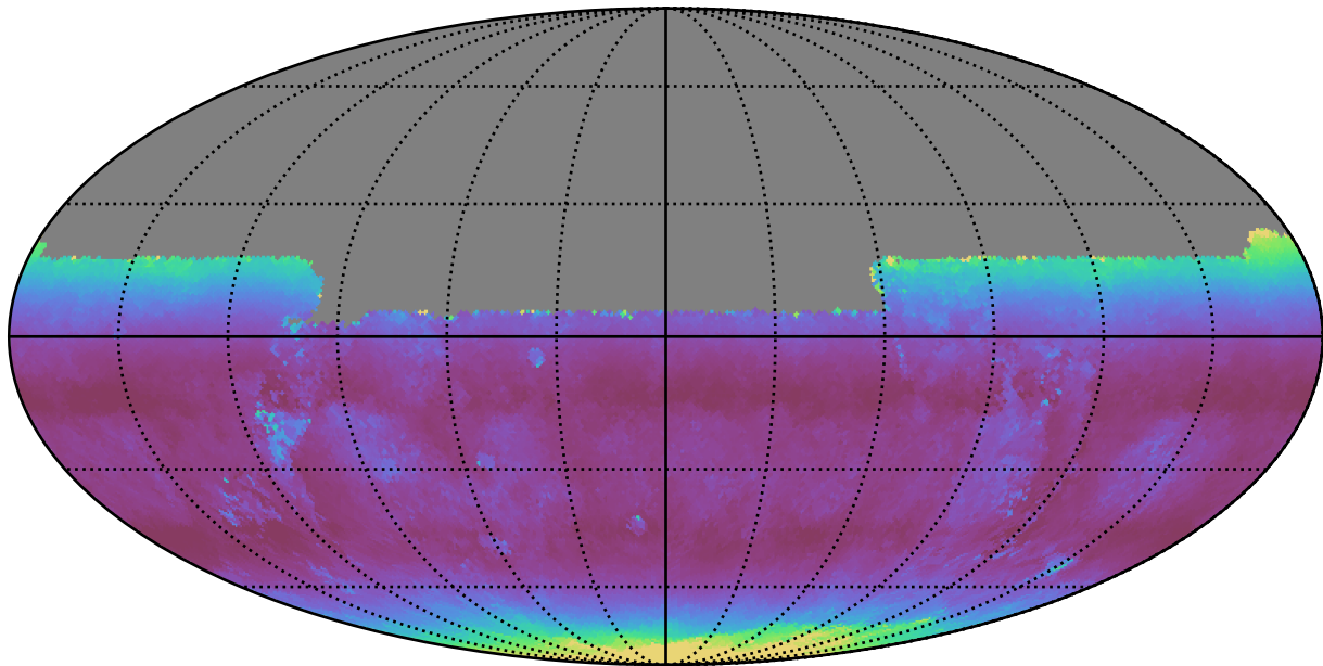
extra_ss_neo4_v3.4_10yrs All sky u band: Median airmass
