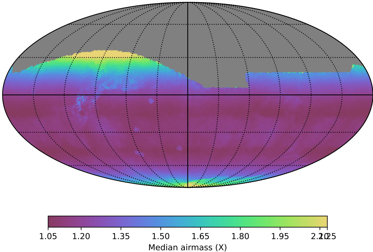
extra_ss_neo4_v3.4_10yrs All sky r band: Median airmass
