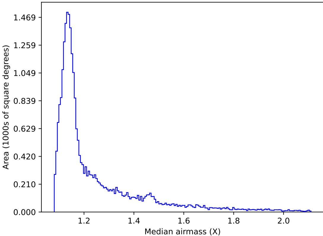
extra_ss_neo4_v3.4_10yrs All sky i band: Median airmass
