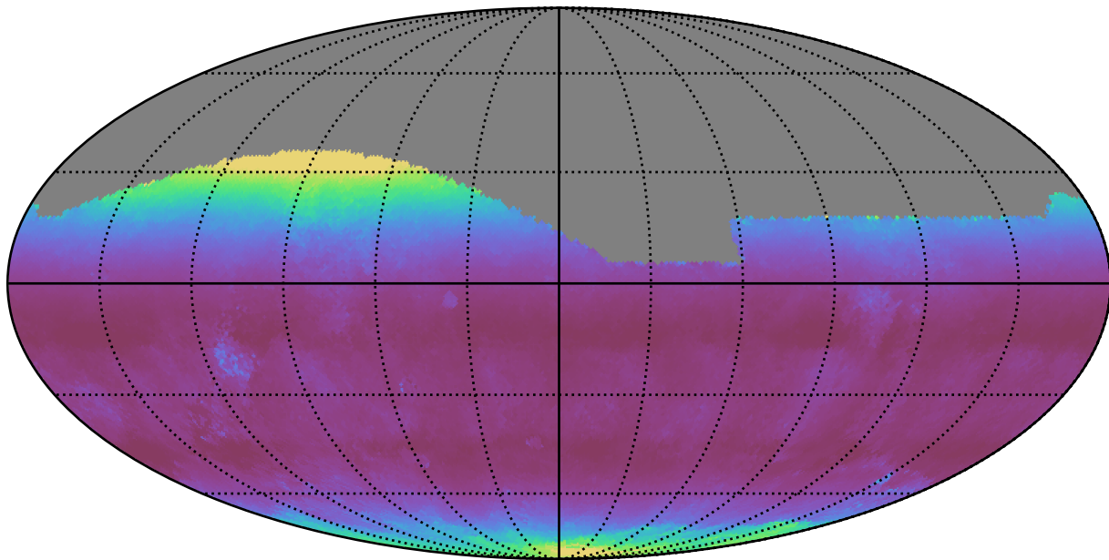
extra_ss_neo4_v3.4_10yrs All sky g band: Median airmass
