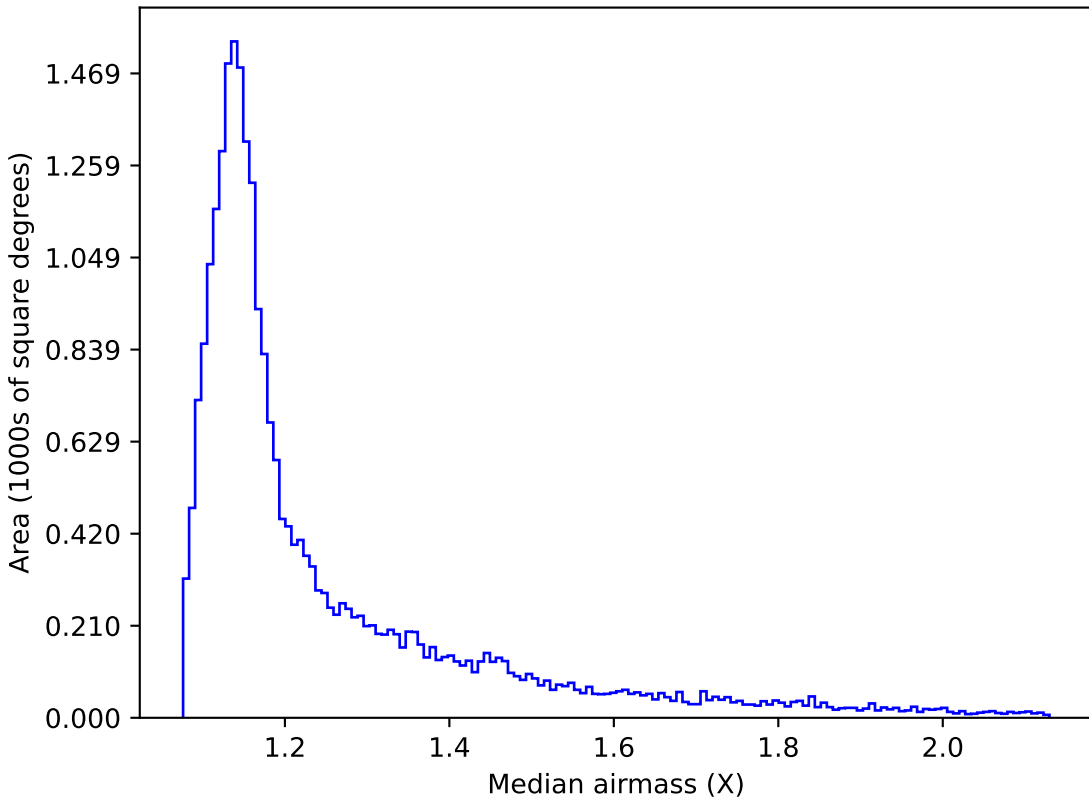
extra_ss_neo4_v3.4_10yrs All sky g band: Median airmass
