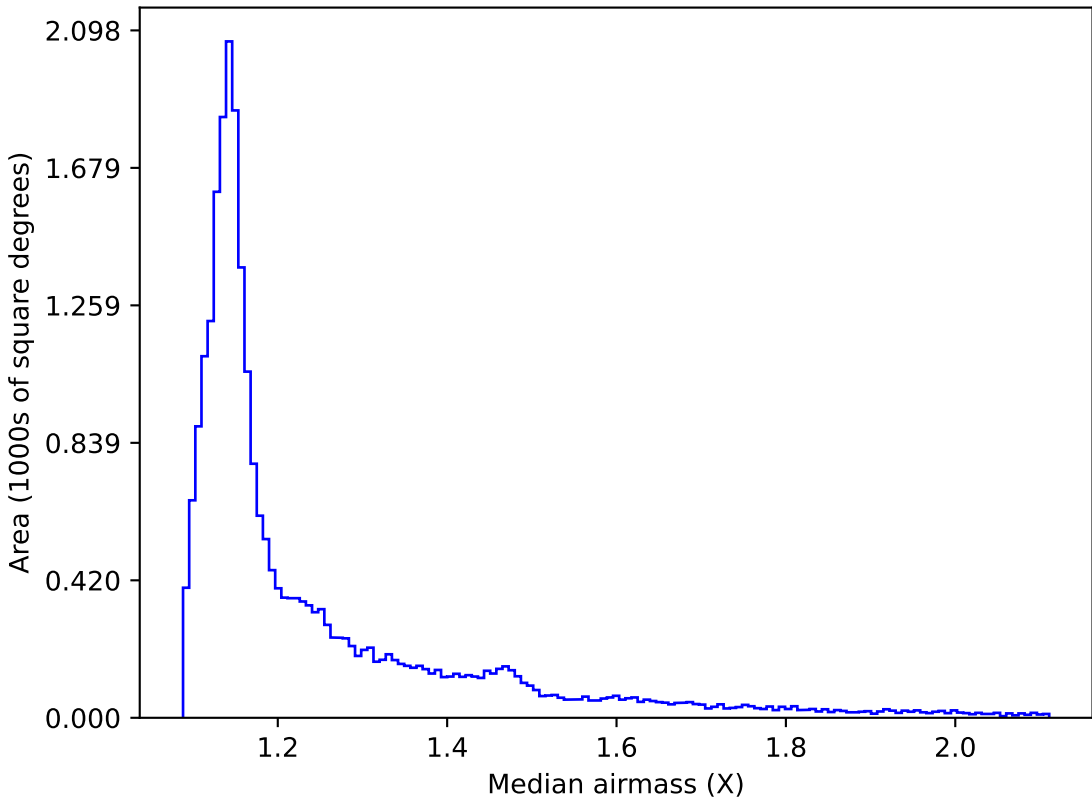
extra_ss_neo4_v3.4_10yrs All sky all bands: Median airmass
