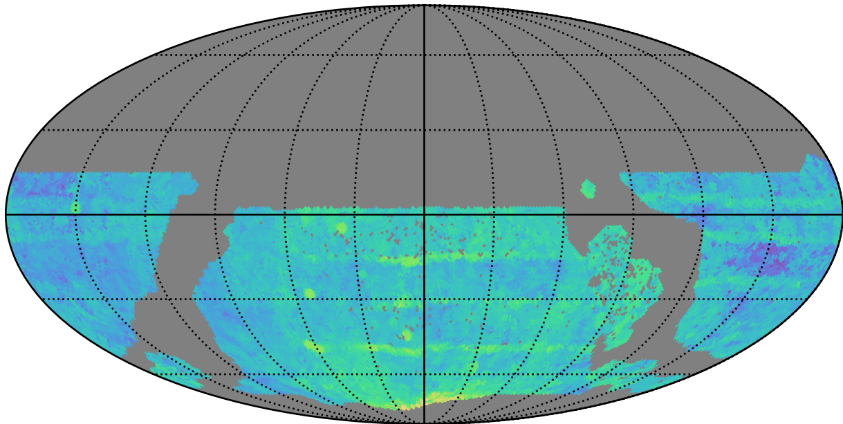
extra_ss_neo4_v3.4_10yrs WFD z band: Median Season Length
