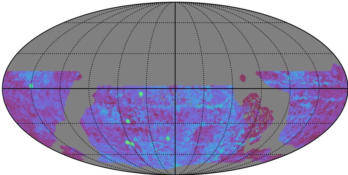
extra_ss_neo4_v3.4_10yrs WFD u band: Median Season Length
