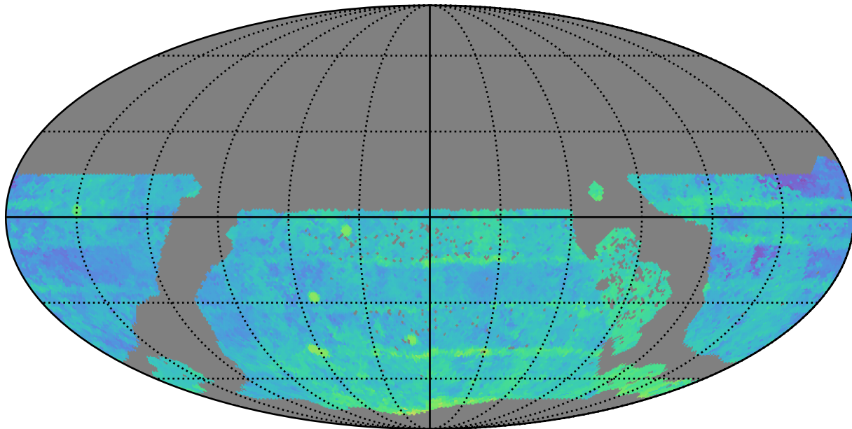
extra_ss_neo4_v3.4_10yrs WFD r band: Median Season Length
