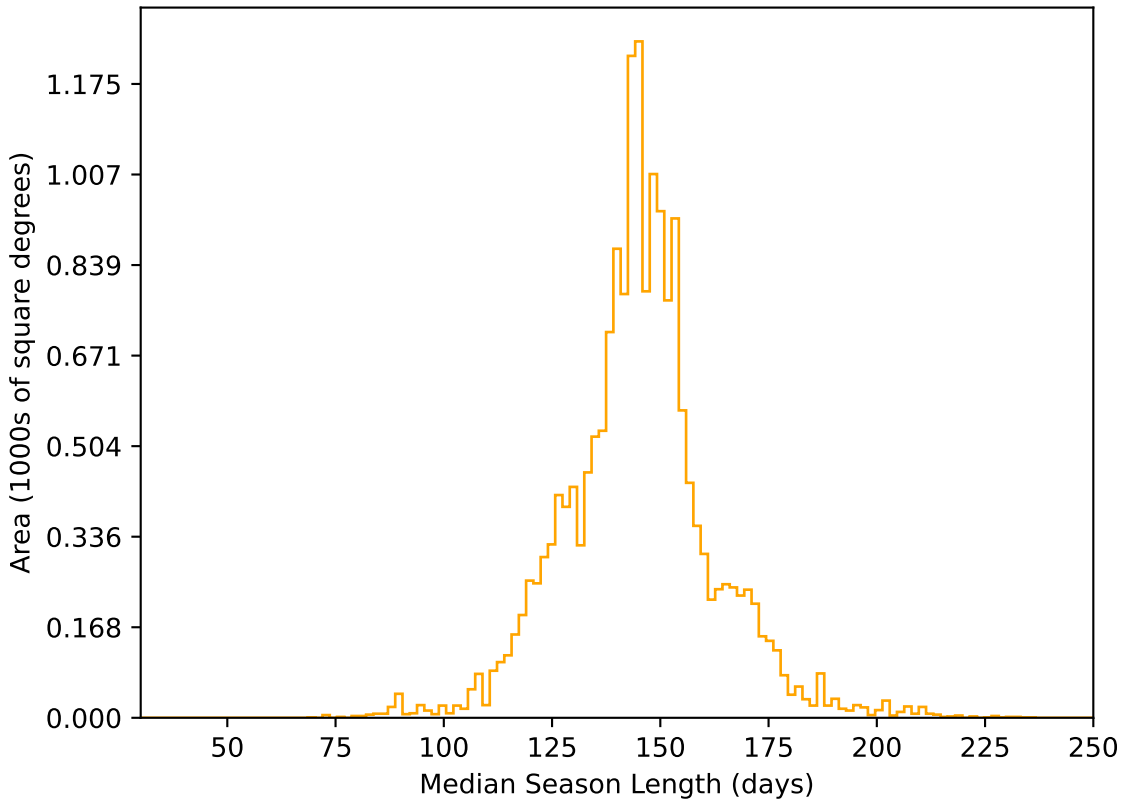
extra_ss_neo4_v3.4_10yrs WFD r band: Median Season Length
