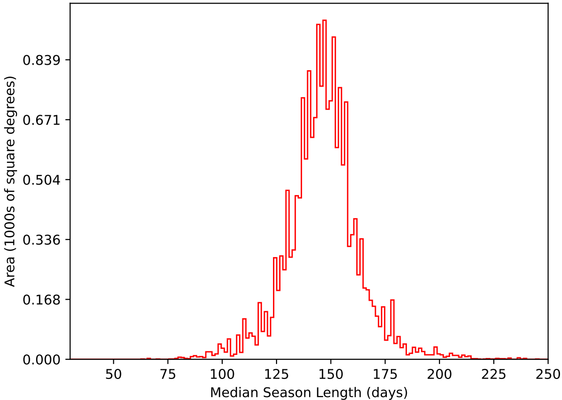
extra_ss_neo4_v3.4_10yrs WFD i band: Median Season Length
