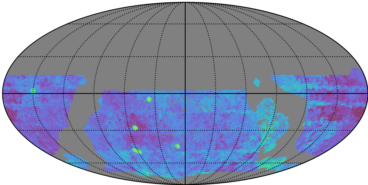
extra_ss_neo4_v3.4_10yrs WFD g band: Median Season Length
