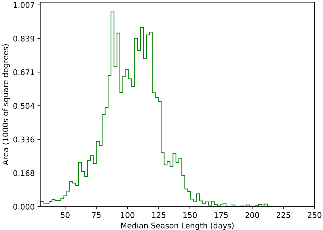
extra_ss_neo4_v3.4_10yrs WFD g band: Median Season Length
