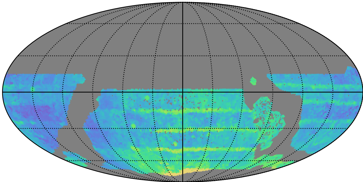
extra_ss_neo4_v3.4_10yrs WFD all bands: Median Season Length
