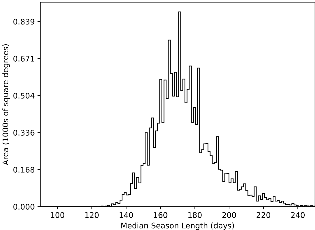
extra_ss_neo4_v3.4_10yrs WFD all bands: Median Season Length
