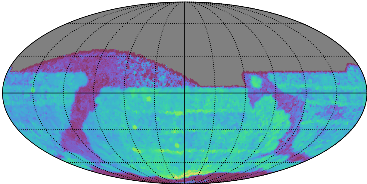
extra_ss_neo4_v3.4_10yrs All sky z band: Median Season Length
