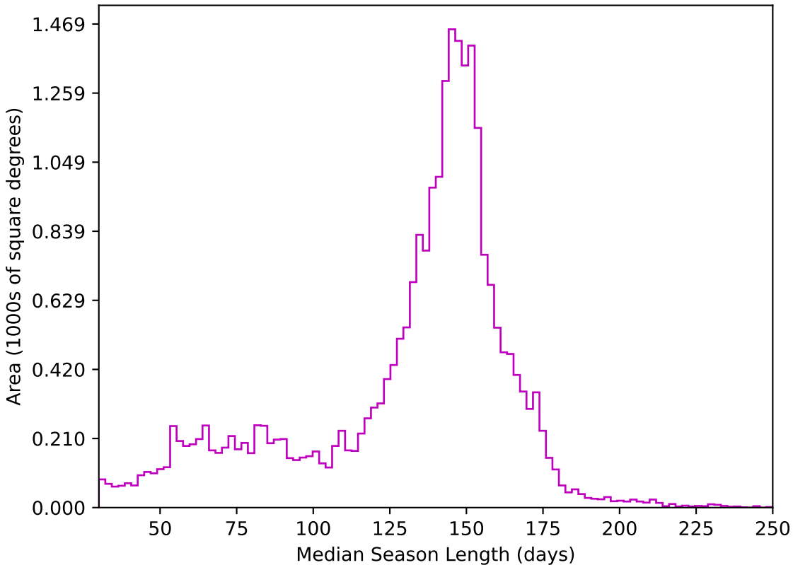
extra_ss_neo4_v3.4_10yrs All sky z band: Median Season Length
