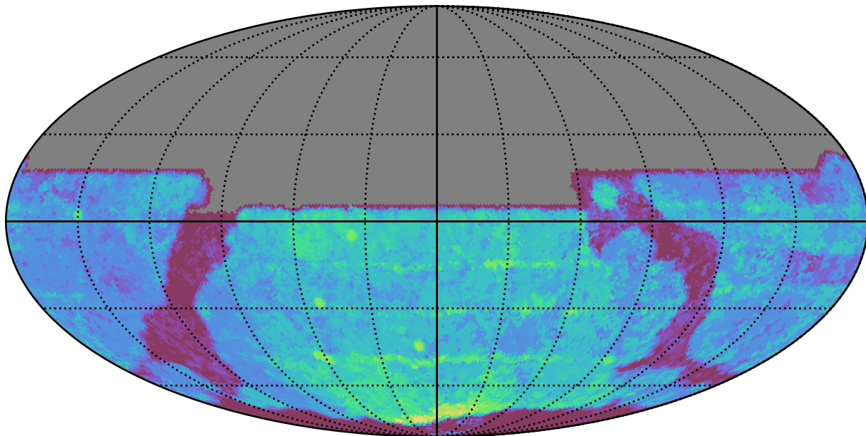
extra_ss_neo4_v3.4_10yrs All sky y band: Median Season Length
