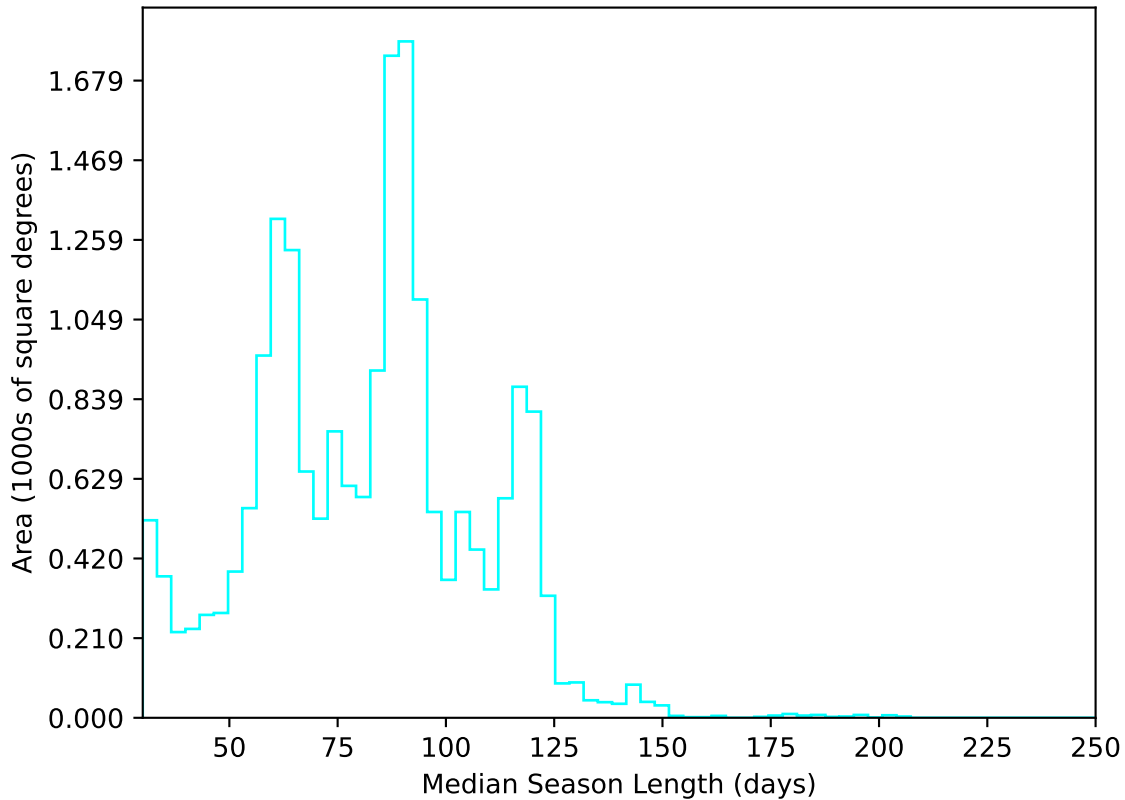
extra_ss_neo4_v3.4_10yrs All sky u band: Median Season Length
