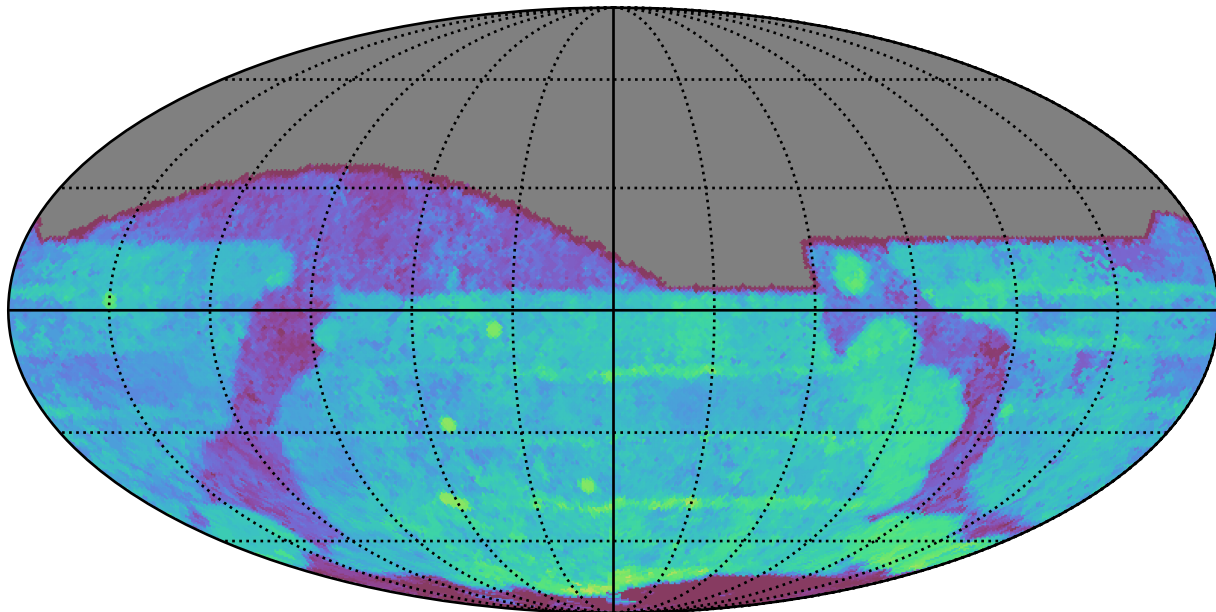
extra_ss_neo4_v3.4_10yrs All sky r band: Median Season Length
