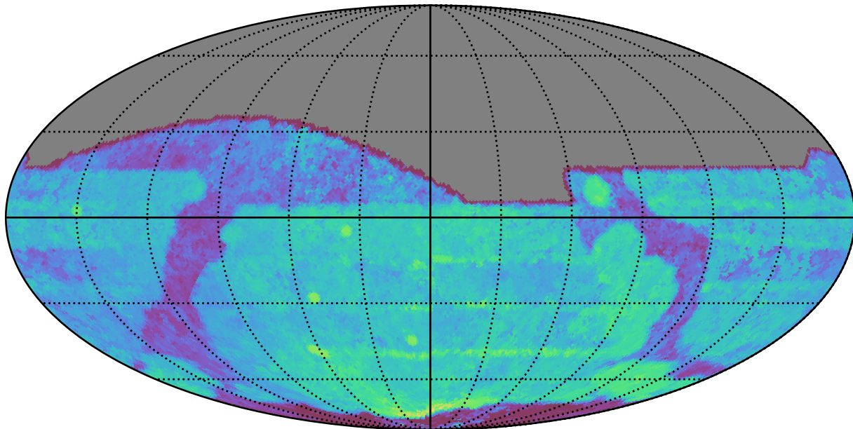
extra_ss_neo4_v3.4_10yrs All sky i band: Median Season Length
