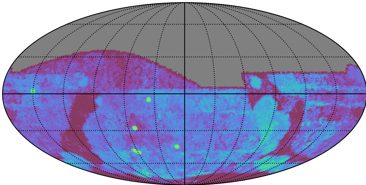
extra_ss_neo4_v3.4_10yrs All sky g band: Median Season Length
