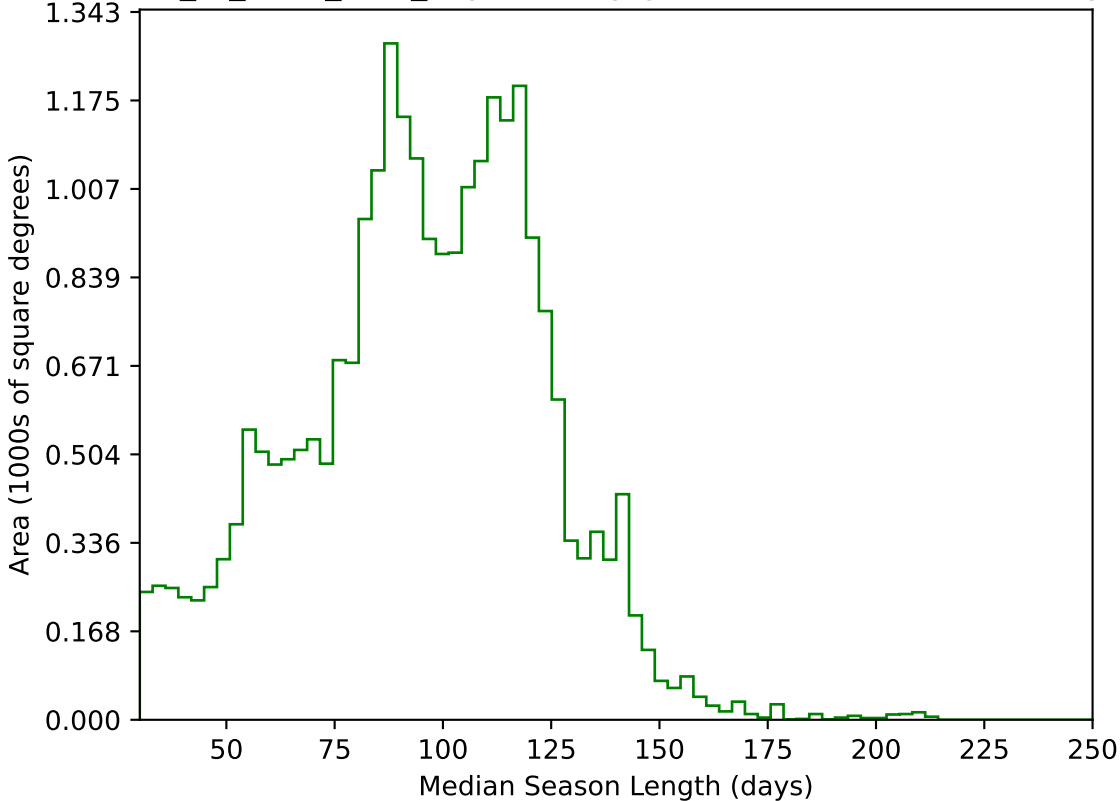
extra_ss_neo4_v3.4_10yrs All sky g band: Median Season Length
