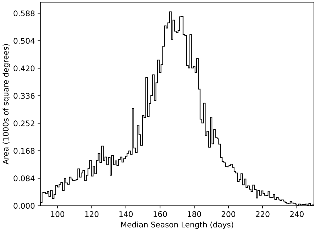
extra_ss_neo4_v3.4_10yrs All sky all bands: Median Season Length
