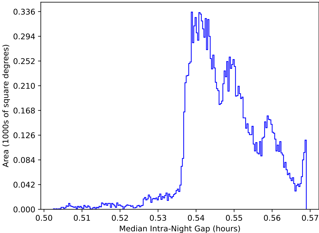
extra_ss_neo4_v3.4_10yrs WFD: Median Intra-Night Gap
