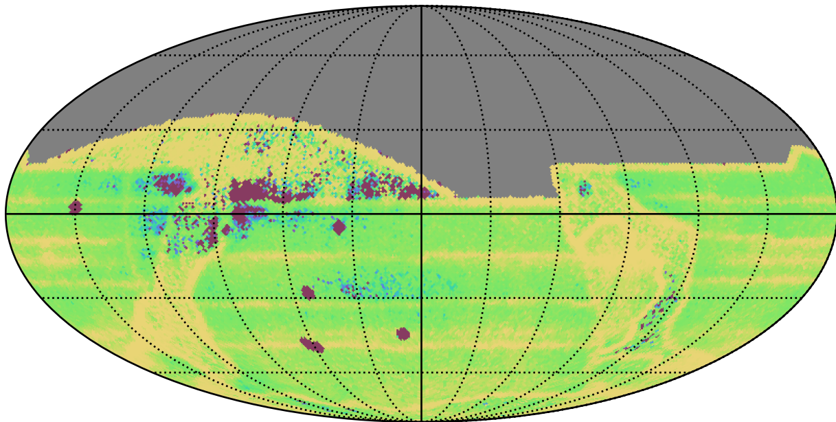
extra_ss_neo4_v3.4_10yrs All sky: Median Intra-Night Gap
