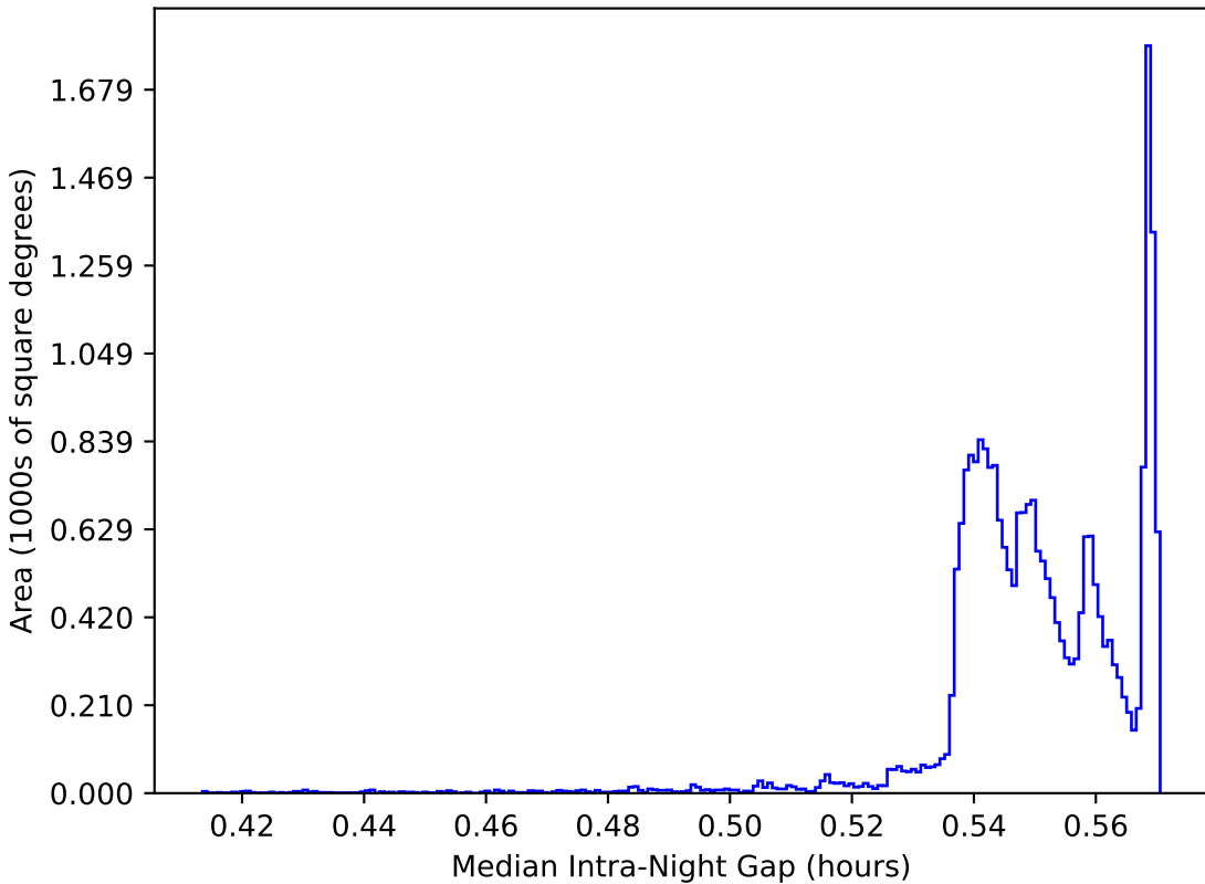
extra_ss_neo4_v3.4_10yrs All sky: Median Intra-Night Gap
