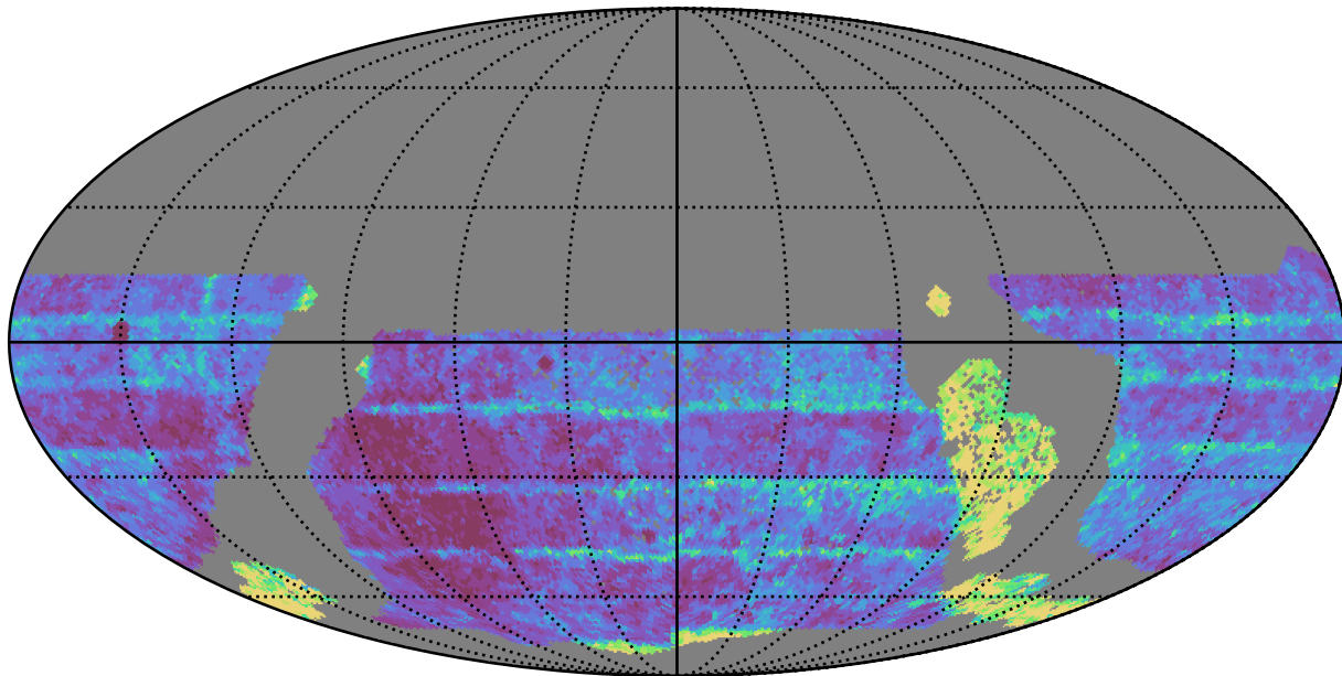
extra_ss_neo4_v3.4_10yrs WFD z band: Median Inter-Night Gap
