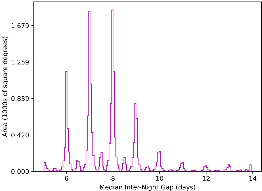
extra_ss_neo4_v3.4_10yrs WFD z band: Median Inter-Night Gap
