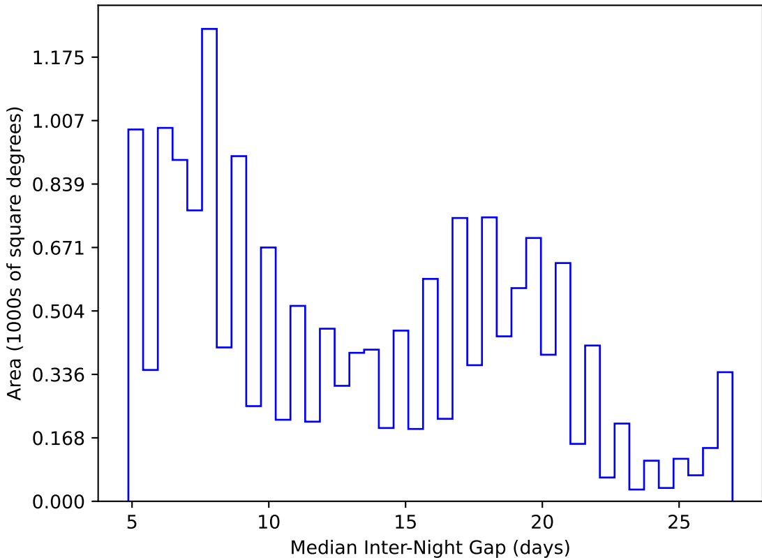
extra_ss_neo4_v3.4_10yrs WFD y band: Median Inter-Night Gap
