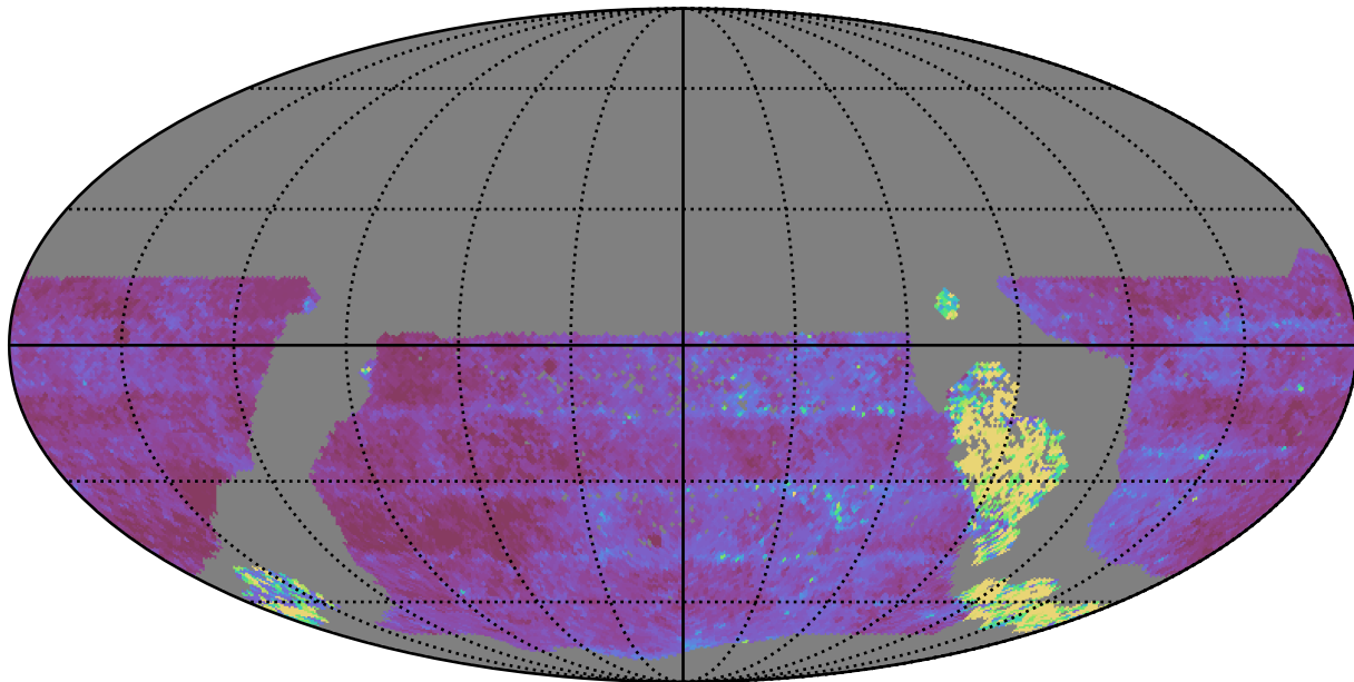
extra_ss_neo4_v3.4_10yrs WFD u band: Median Inter-Night Gap
