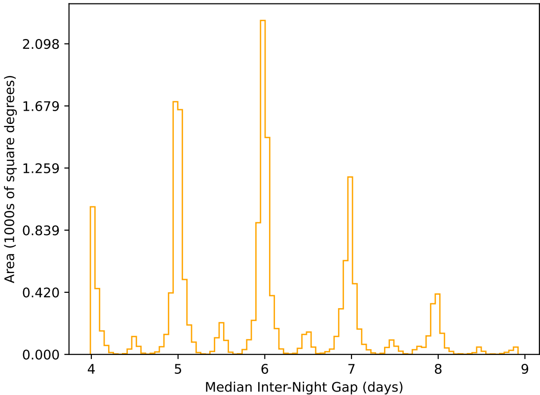
extra_ss_neo4_v3.4_10yrs WFD r band: Median Inter-Night Gap
