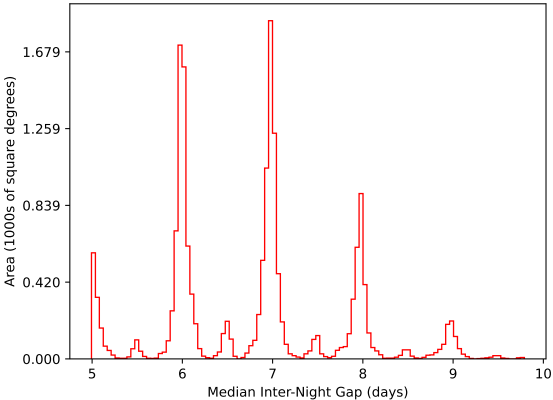
extra_ss_neo4_v3.4_10yrs WFD i band: Median Inter-Night Gap
