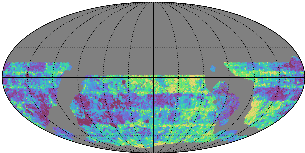
extra_ss_neo4_v3.4_10yrs WFD g band: Median Inter-Night Gap
